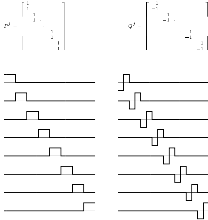
Figure 17 The piecewise-constant B-spline (Haar) scaling functions and wavelets for j = 3 .
