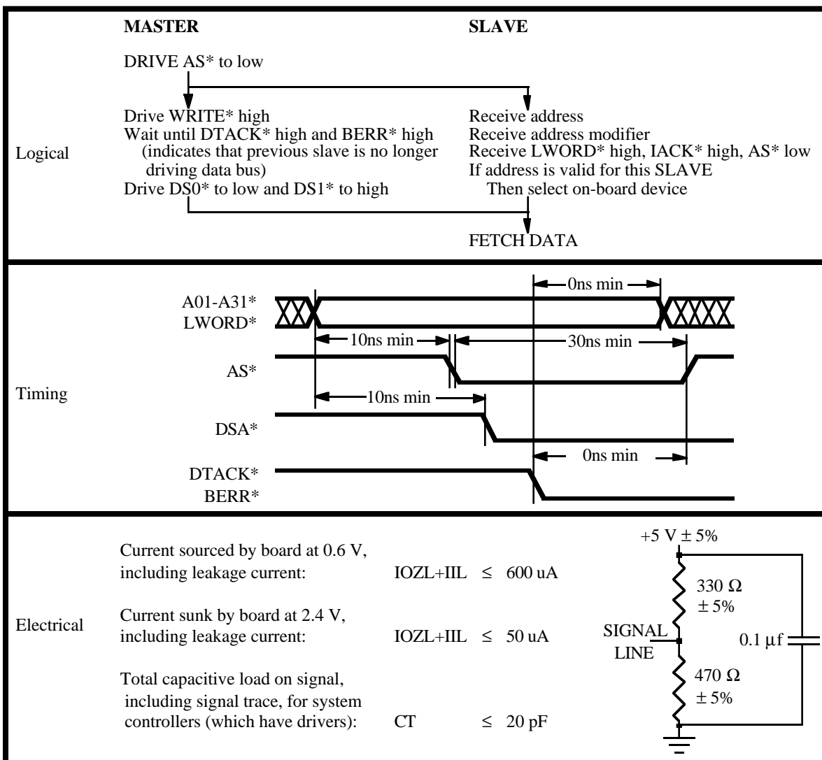
Figure 1. A communication protocol can be considered to have three levels: electrical, timing, and logical. Examples in this figure adapted from the VMEbus specification [VMEbus85].
