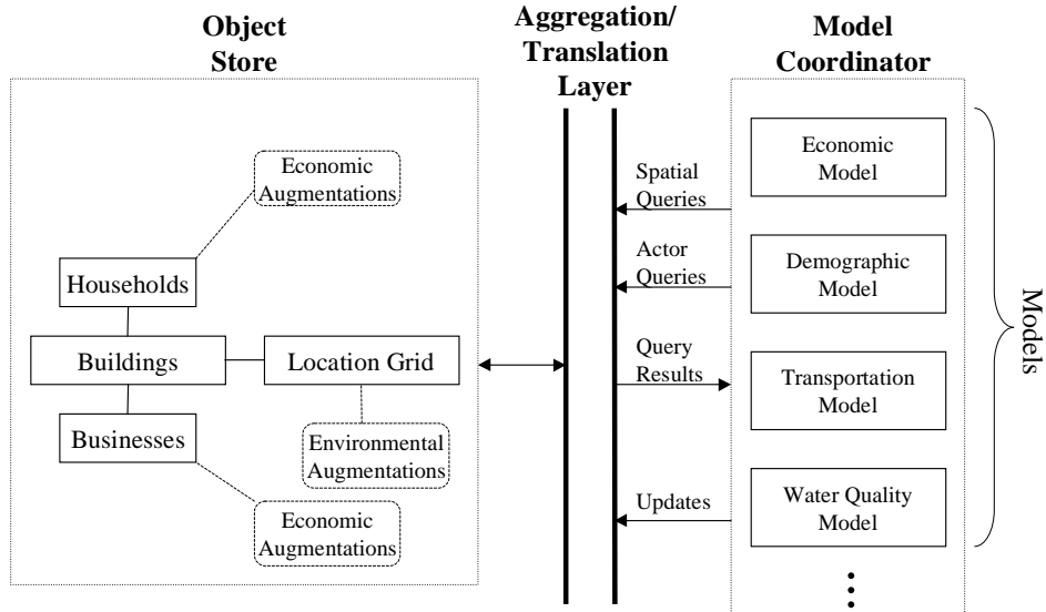
Figure 1: UrbanSim architecture
