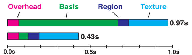
figure 3.3: Rendering profile for a single frame, before and after basis optimizations. “Overhead” includes OpenGL state setup and culling of rendering passes. “Basis” includes rendering of basis functions into alpha. “Region” includes rendering region geometry. “Texture” includes loading texture images. Times for the various stages are approximately additive, but not completely due to some pipeline parallelism.
