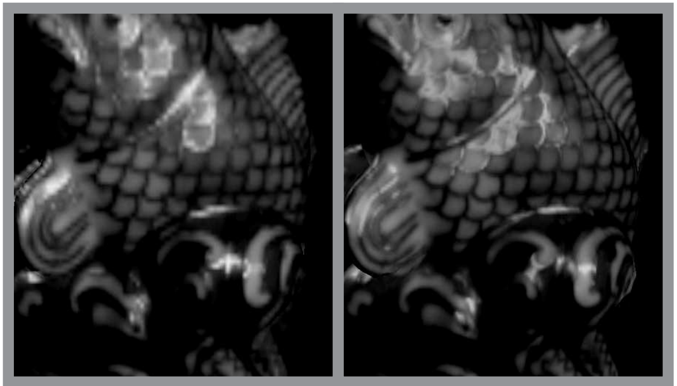
Image B: Lumigraph, 238x238 UV, 7x7 ST Insufficient surface detail resolution
