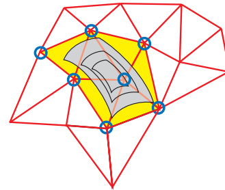
figure 3.2: Reversed direction mesh and region geometry seen from the camera. Only vertices incident on traversed triangles are contributing directions.
