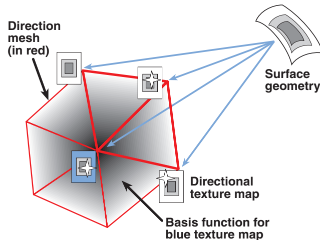
figure 2.2: Texture maps are associated with directions. Directions are arranged in a direction mesh, and each has a corresponding basis function.
