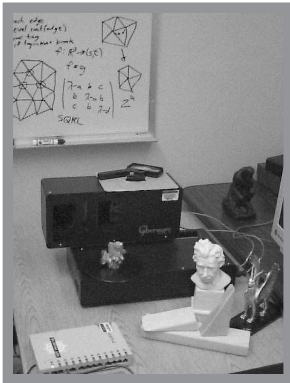
Figure 5.1: Cyberware Model 15 laser range scanner
