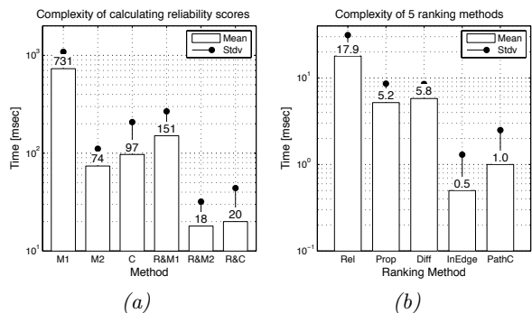
Figure 8: (M1: Monte Carlo 10000 simulations, M2: Monte Carlo 1000 simulations, R: Reduction of graph, C: Closed solution)
