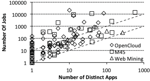
Figure 5: The number of distinct applications and the number of jobs per user. Each point corresponds to one user. The reference lines represent y = x and y = 10x respectively. Users above y = 10x line run the same job more than 10 times. All three clusters have a good mix between exploratory and repetitive applications. Many users executed only a single application.
