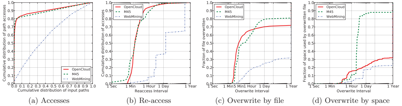
Figure 11: Distribution of various access patterns. (a) shows the distribution of access frequency of data paths; (b) shows the distribution of re-access frequency of input and output data; (c) shows the distribution of time intervals between output data with the same data paths; (d) shows the distribution of space used by overwritten data within different time intervals.
