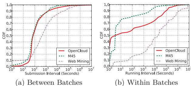
Figure 8: Distribution of the submission interval between successive batches for the same user, and running interval between jobs within a batch. Jobs that share a data dependency (as defined in Sec.3.1) are considered to be in the same batch.
