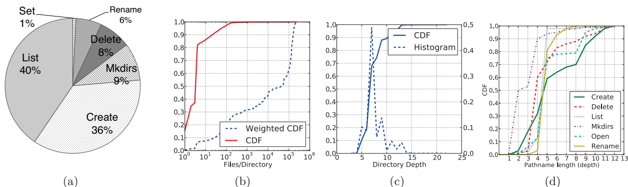
Figure 12: Namespace statistics in OPENCLOUD: (a) Distribution of HDFS NameNode operations except open in OPENCLOUD; (b) CDF and Weighted CDF of directories by count of files; (c) Distribution of files by directory depth; (d) Distribution of HDFS NameNode operations by length of accessed pathname.
