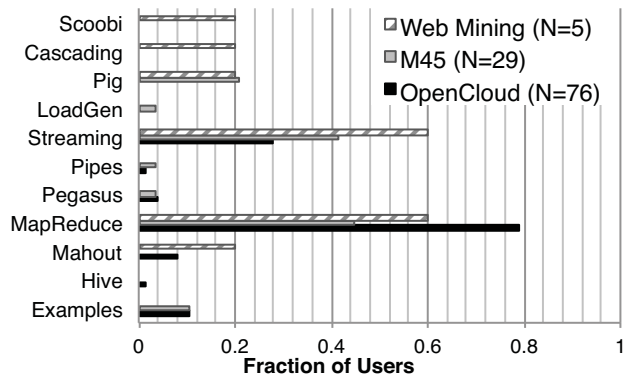
Figure 3: Fraction of users per application type.
