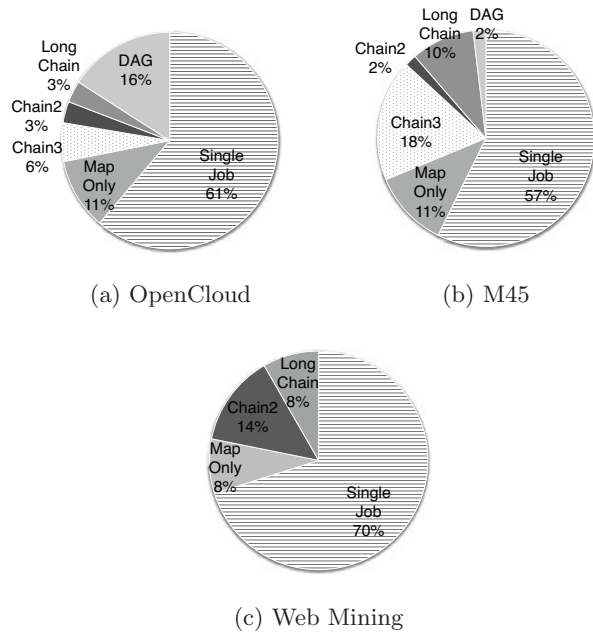
Figure 1: Distribution of job structures in three workloads.
