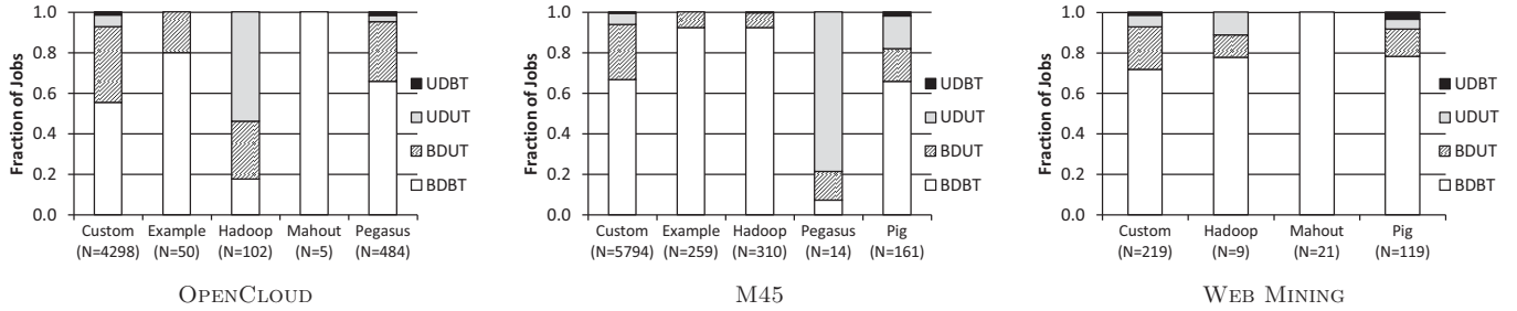
Figure 15: Distribution of map runtime with respect to # of input records per application. N is the number of successful jobs that run map functions in each category. The labels indicate the category: (U)BD(U)BT stands for (un)balanced input data, (un)balanced runtime.
