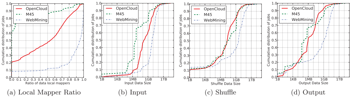
Figure 10: (a) Distribution of jobs with different ratios of data local mappers; (b)-(d) Distribution of per-job data size for the input, shuffle and output phase.
