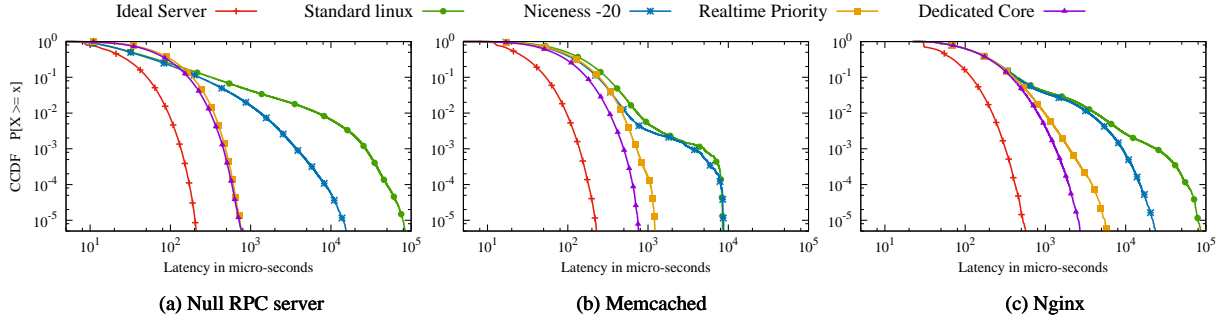
Figure 5: The effect of background processes on tail latency. For this experiment, we disabled all but a single core on a single CPU, and we loaded the server at 80-85% utilization.
