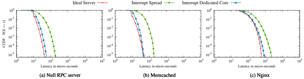
Figure 8: Impact of directing interrupts to a specific core versus spreading across all cores. In the first case, interrupts are spread across all cores, whereas in the second case interrupts go to a dedicated core and application threads run on remaining cores.
