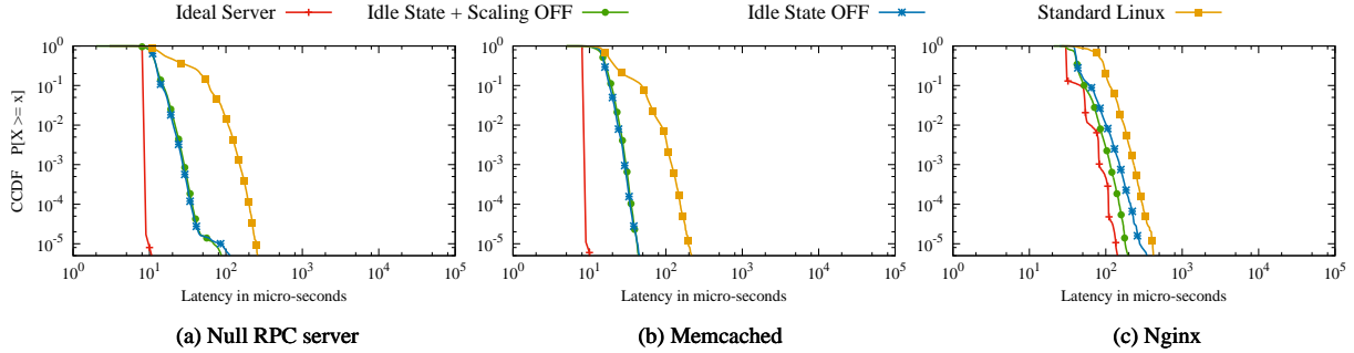
Figure 10: Impact of power saving optimizations on tail latency at low (10%) utilization.
