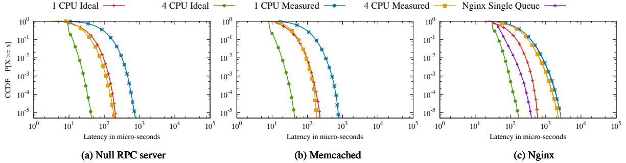
Figure 7: Tail latency improvement as we scale to multiple cores. 4 cores at 75%-80% utilization.
