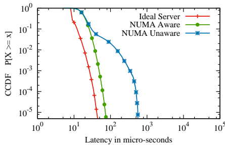
Figure 9: Impact of NUMA aware memory allocation in Memcached running on 8 cores (across NUMA nodes) at 75% utilization.
