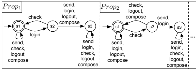
Fig. 5. Property instances mined by InvariMint from the log in Figure 2(a), based on property types in Figure 4(a). Prop_1 represents “event login can be immediately followed by an event from set \{\text{check}\} ”. Prop_2 represents “event check can be immediately followed by an event from set \{\text{check}, \text{logout}, \text{compose}\} ”.
