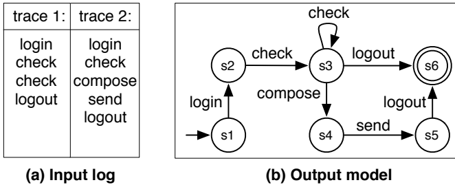
Fig. 2. (a) An example log of an email client. (b) The model inferred by SimpleAlg (Figure 3).
