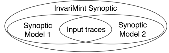
Fig. 14. The relationships between the language of the model derived using an InvariMint formulation of Synoptic, the language of the Synoptic model for the same input traces, and the input traces.
